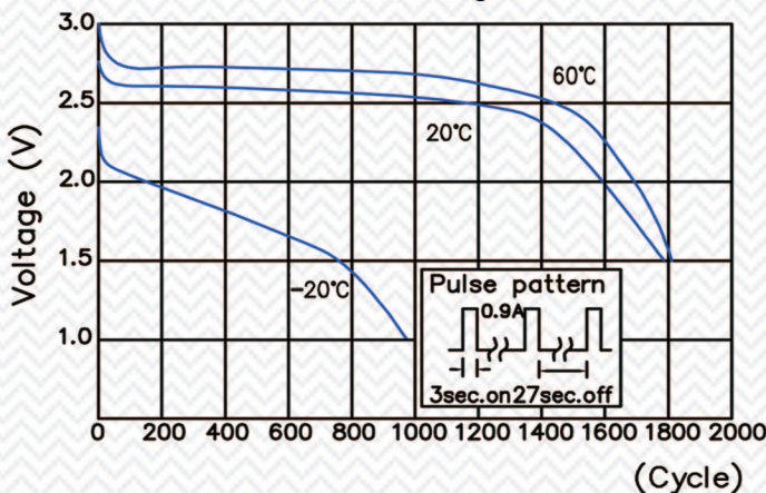
Pulse Discharge
