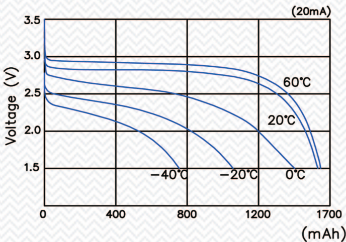
20mA Discharge
