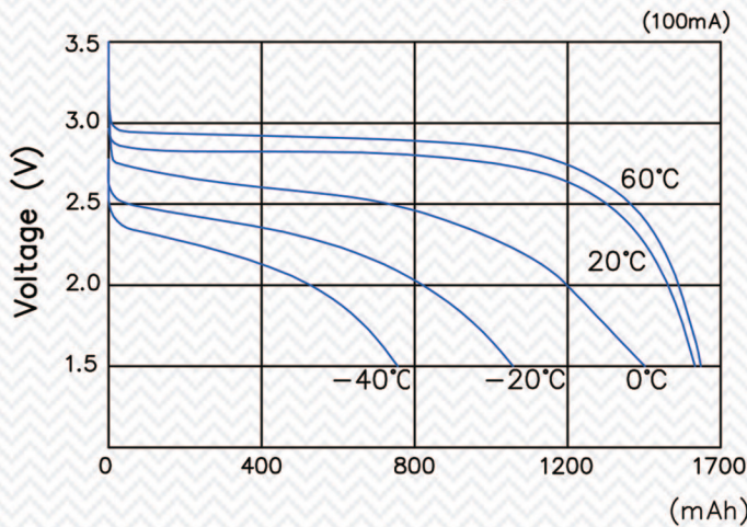
100mA Discharge
