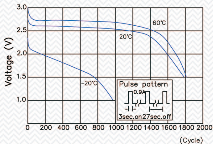
Pulse Discharge
