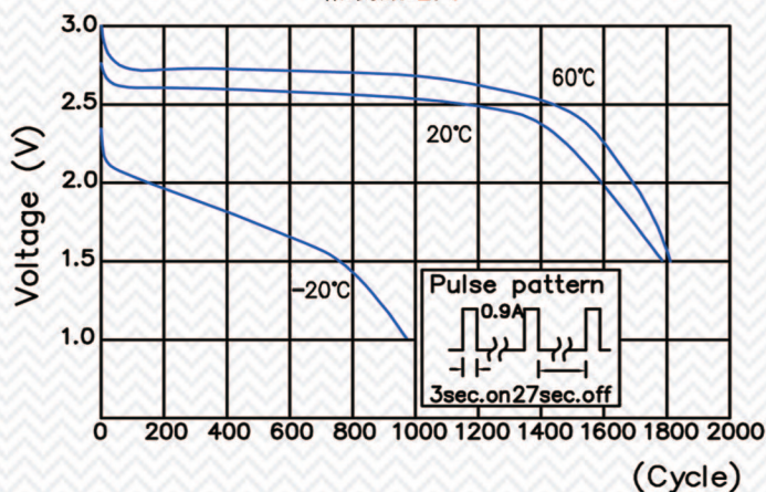
脈衝放電圖
