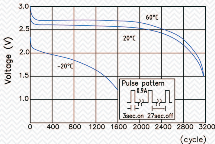
脈衝放電圖
