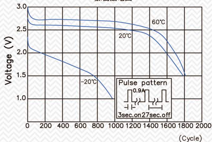
脈衝放電圖
