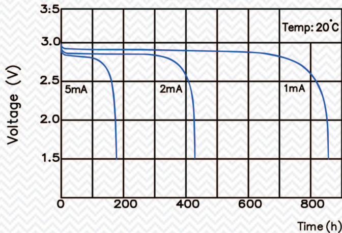
脈衝放電圖
