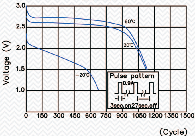
脈衝放電圖
