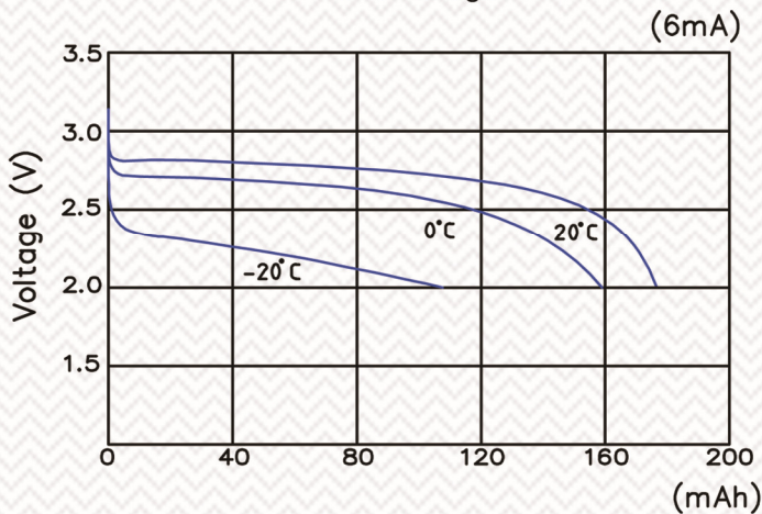
6mA Discharge
