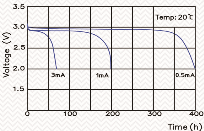
Pulse Discharge
